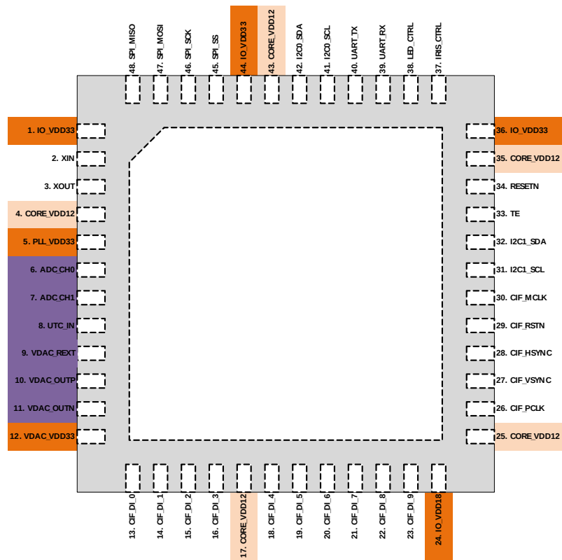
Figure 2 PI4009K Package View
